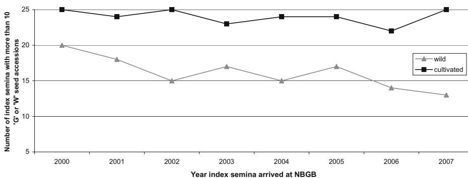
Graph 2 The number of seed lists comprising of wild 'W' and garden 'G' collected accessions from the 25 seed lists assessed in each year between 2000 & 2007. Years refer to the arrival date of the seed list in the NBGB, not the collection date of material.
