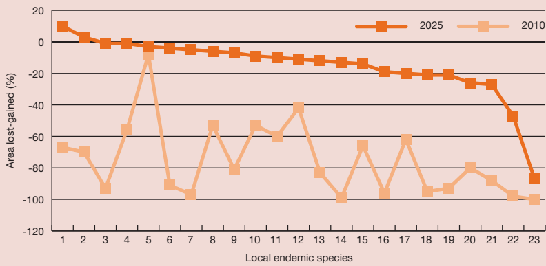
Figure 2. Changes in potential distribution after climate change scenarios for different local and regional endemic species of Cactaceae in the Tehuacan-Cuicatlán Biosphere Reserve
